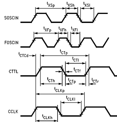
FIGURE 4-8. Clock Waveforms
