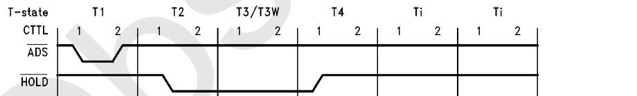
FIGURE 3-20. Spaced Memory Transaction, Two Tidles after T4
