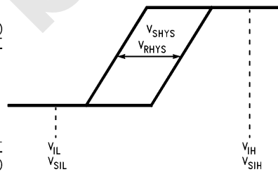
FIGURE 4-7. Input Hysteresis
