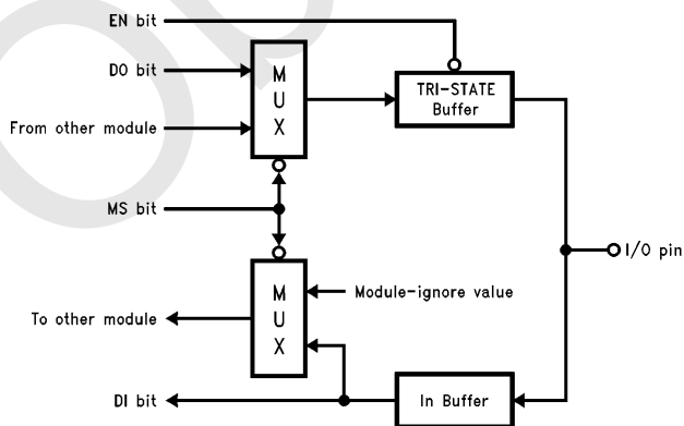
FIGURE 2-25. Port C
