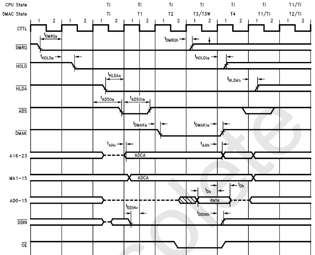
FIGURE 4-16. DMA Read Transaction (DIR = 0)
