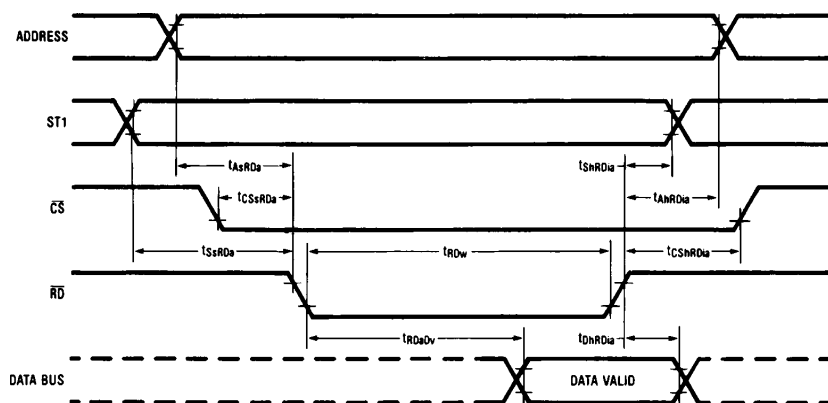
FIGURE 4-3. READ/INTA Cycle
